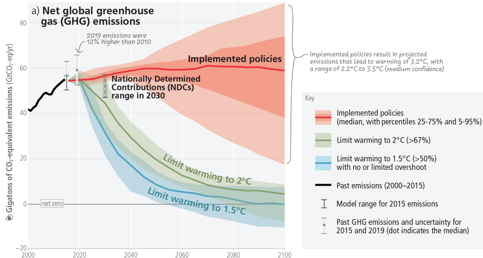
Figure SPM.5a
