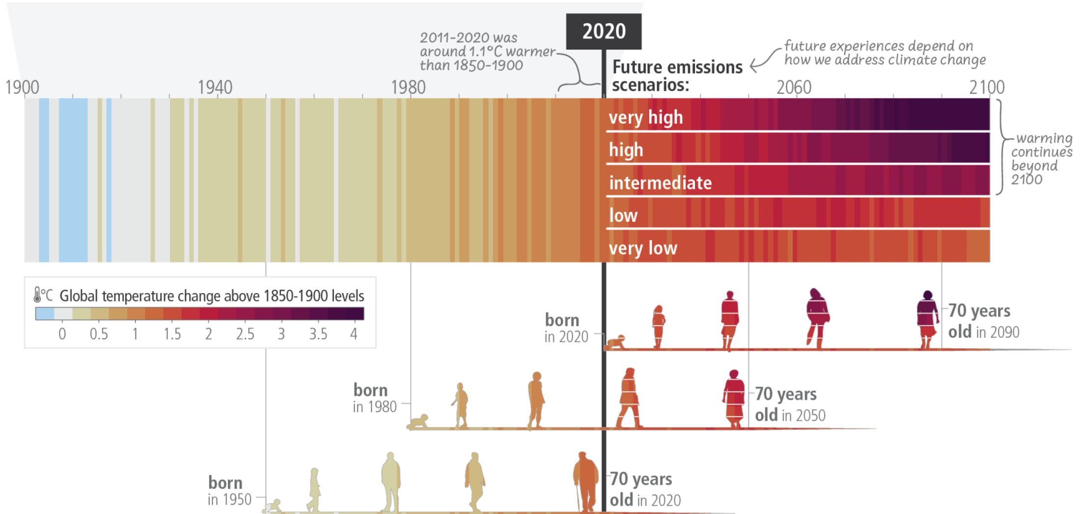
Figure SPM.1c
